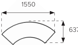
Quadrant Inner High 1550W 637D 600H
