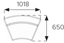
Rotunda Wide Curve (LB) Inner Segment 551/1018W 650D 450/720H
